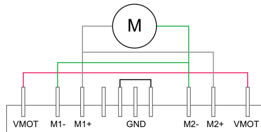
FIGURE 4. XDC2xxxS wiring diagram
