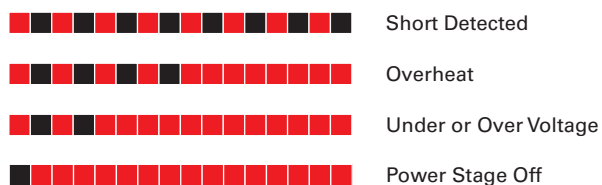
FIGURE 8. Exception or Fault Flashing Patterns
