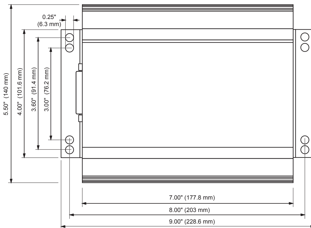
FIGURE 10. XDC2xxx top view and dimensions
