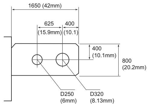
FIGURE 18. High Current copper bar connectors
