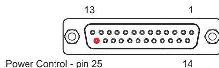
FIGURE 4. Main Connector pin locations
