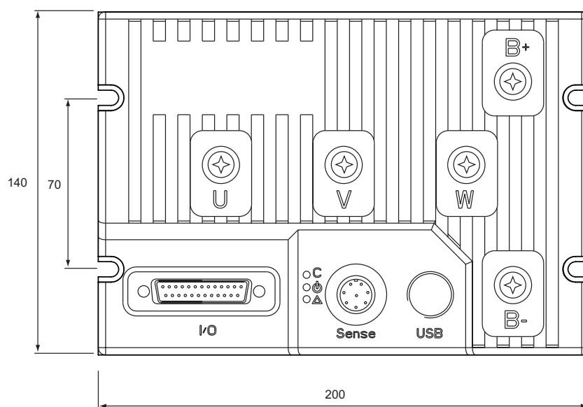
FIGURE 10. RGIM18xx top view and dimensions
