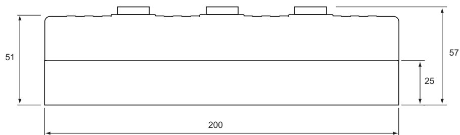
FIGURE 11. RGIM18xx side view and dimensions
