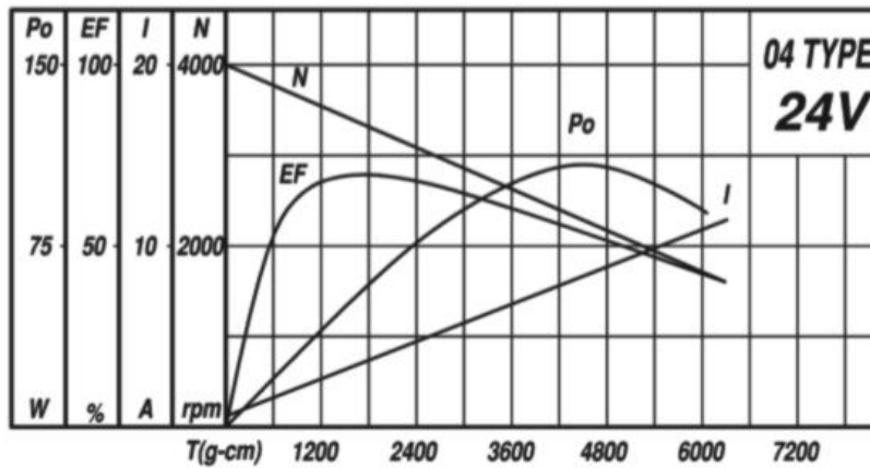
ML-52-12 Motor Specs No Gear Reduction
