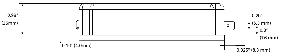
FIGURE 13. MBL1xxx side view and dimensions
