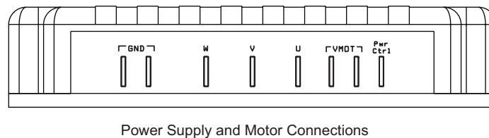
FIGURE 2. MBL1xxx rear view
