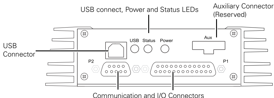
FIGURE 11. Front Controller Layout
