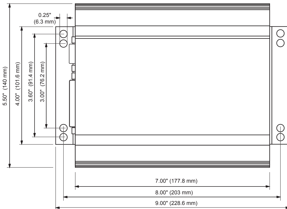
FIGURE 18. HDC24xx top view and dimensions
