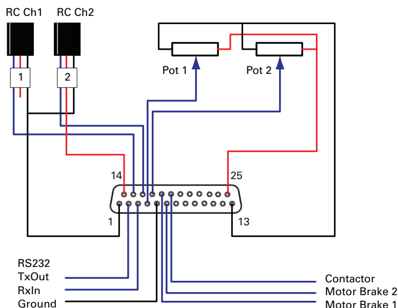
FIGURE 14. Factory default pins assignment
