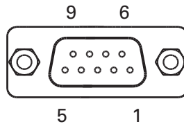
FIGURE 13. Secondary Connector pin locations
