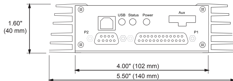
FIGURE 17. HDC24xx front view and dimensions
