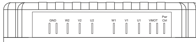
FIGURE 2. FIM2360 rear view
