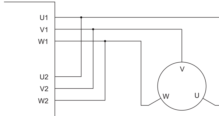
FIGURE 4. Single Channel wiring diagram
