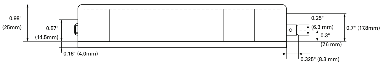
FIGURE 11. FIM2360 side view and dimensions
