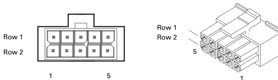
FIGURE 6. Encoder connector
