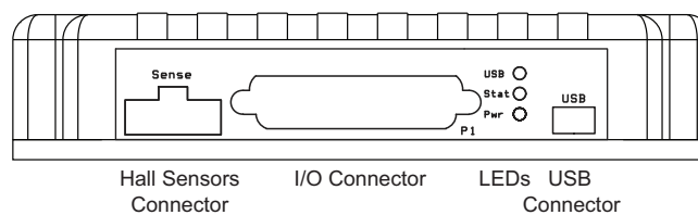
FIGURE 1. FIM2360 front view
