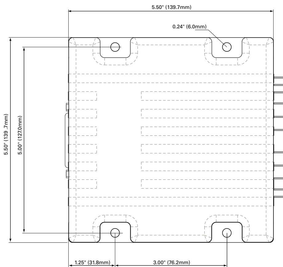
FIGURE 12. FIM2360 top view and dimensions
