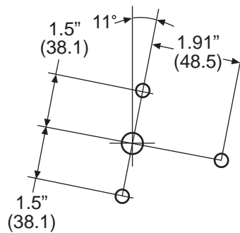
Mounting pattern
