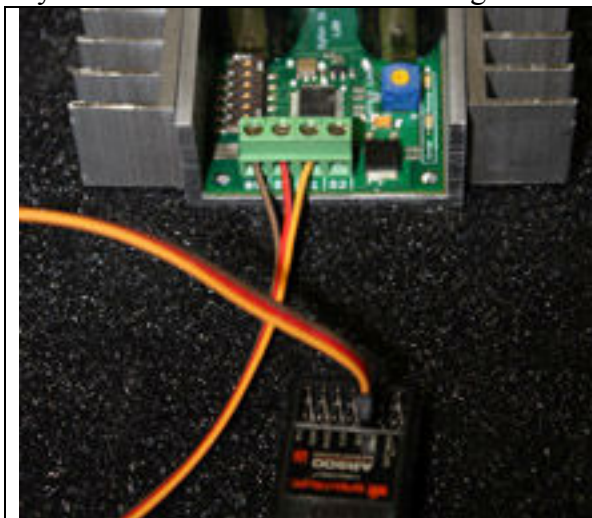
Figure 5.1: R/C connection
