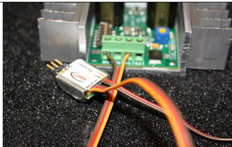
Figure 5.2: R/C with a ParkBEC
